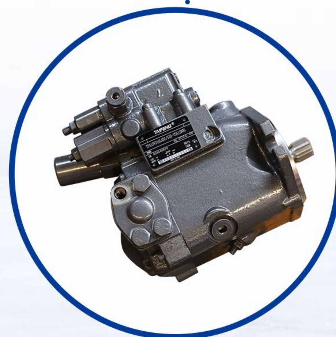
Load Sensing Variable Displacement Piston Pump
